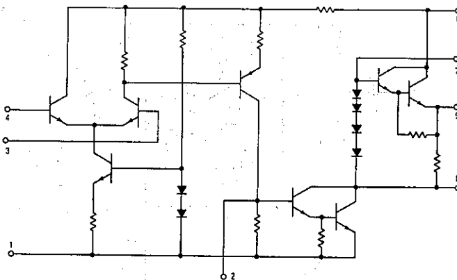
FIGURE 1 – CIRCUIT SCHEMATIC
