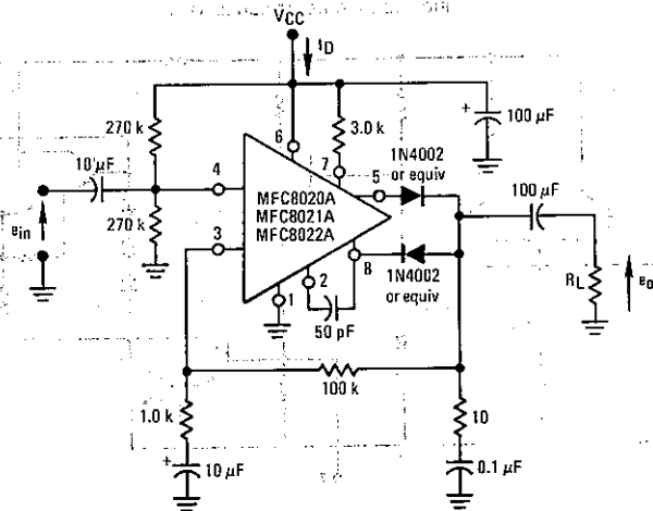
FIGURE 2 - TEST CIRCUIT
