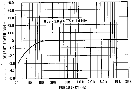
FIGURE 11 — FREQUENCY RESPONSE
