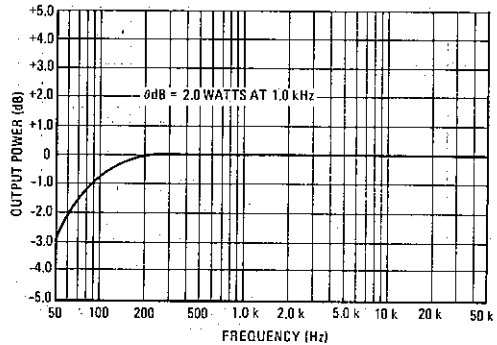
FIGURE 6 - FREQUENCY RESPONSE
